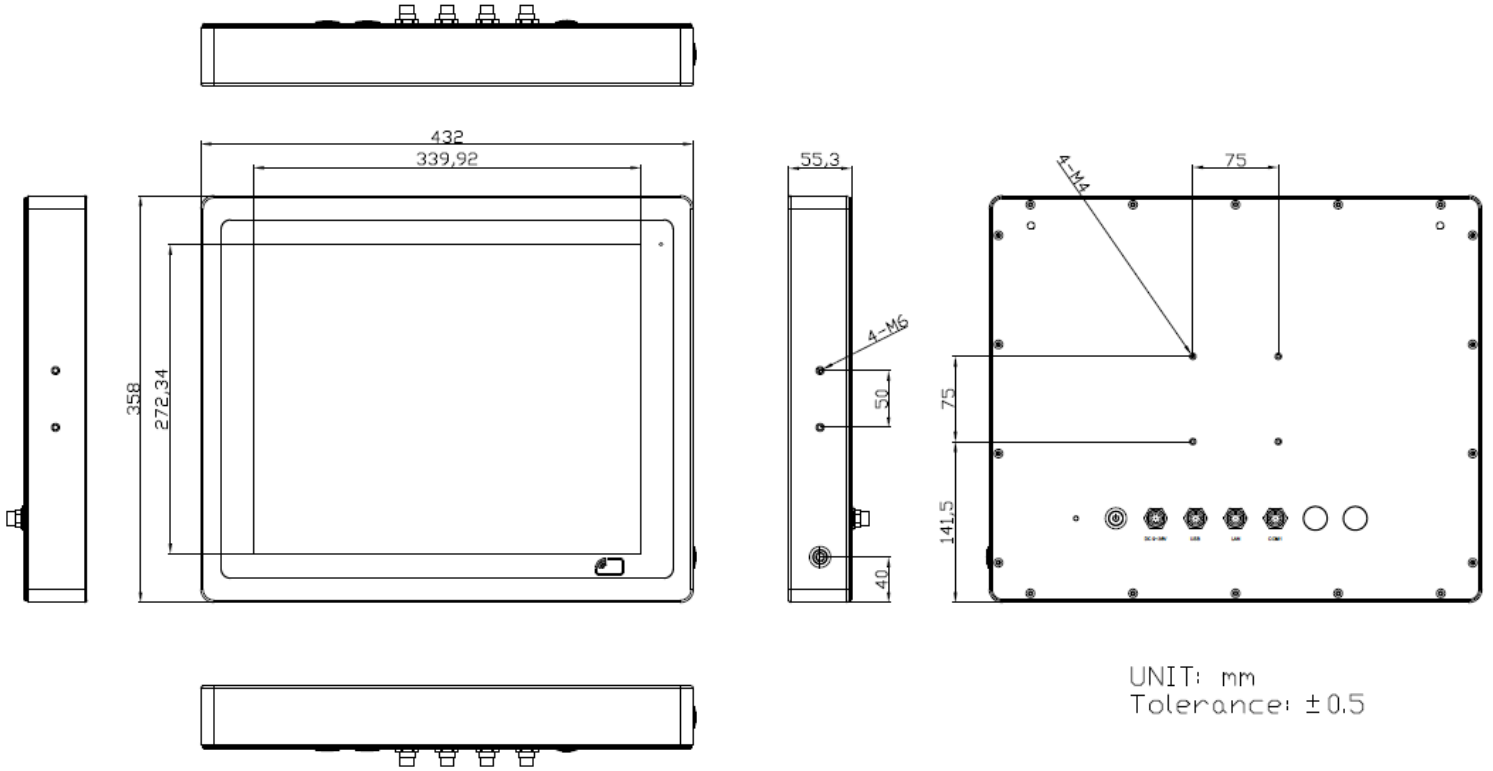
Figure 1.5: Dimensions of EX-91917V
