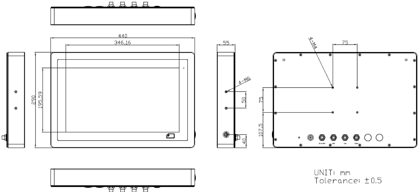
Figure 1.4: Dimensions of EX-91916V
