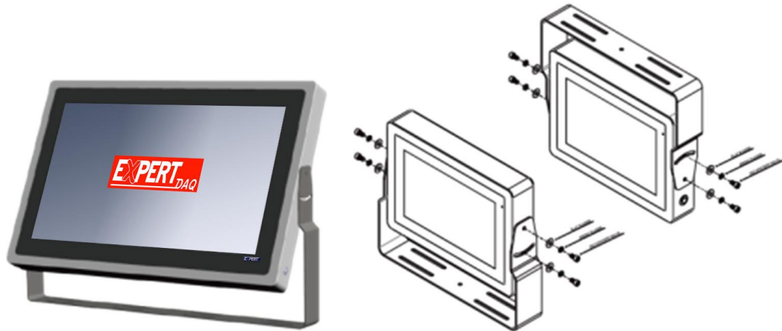
Figure 1.11: Yoke mounting of EX-919xxV Series
