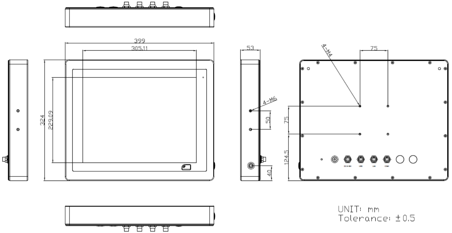
Figure 1.3: Dimensions of EX-91915V
