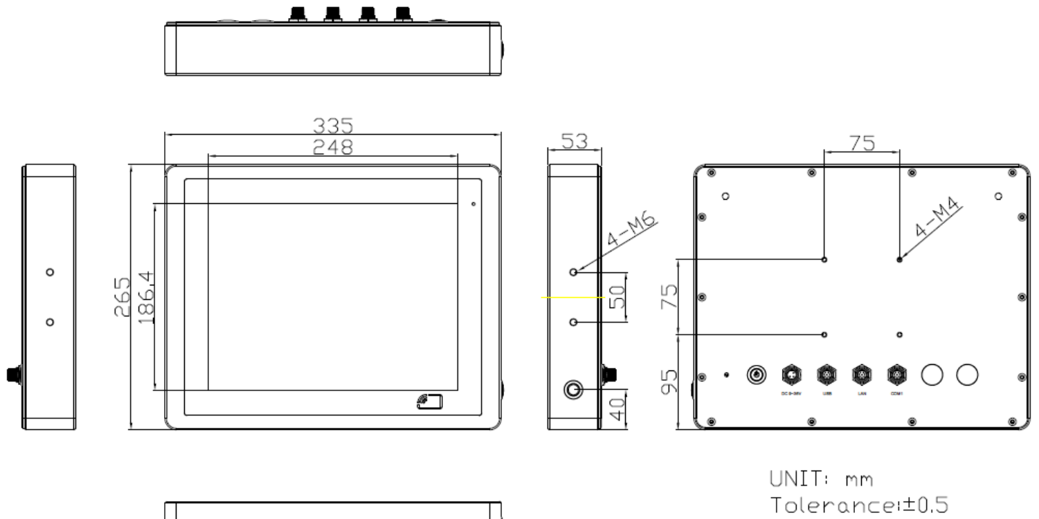
Figure 1.1: Dimensions of EX-91910V
