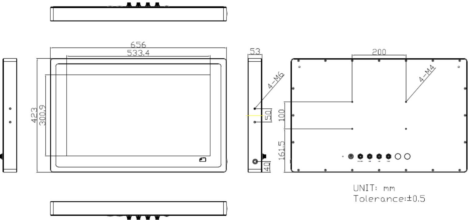
Figure 1.8: Dimensions of EX-91924V
