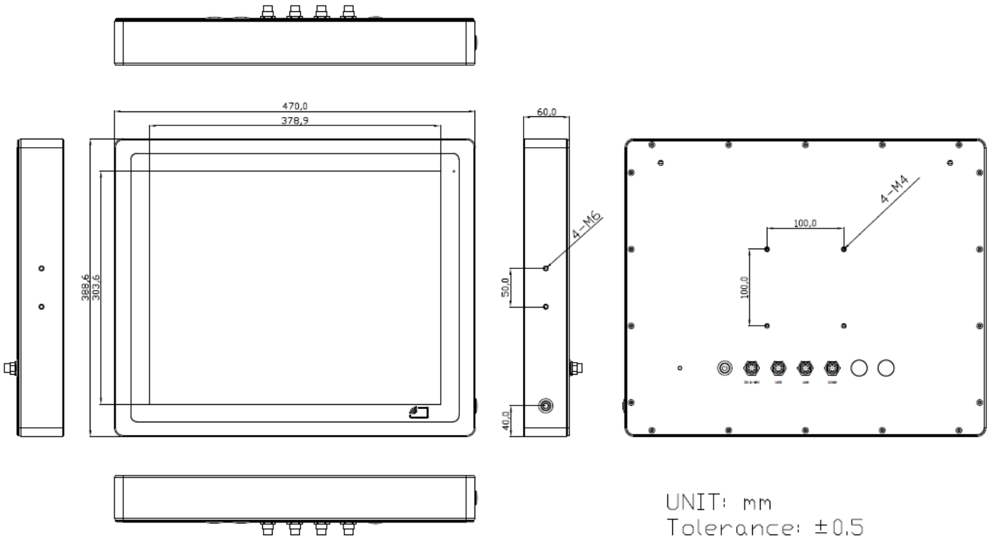
Figure 1.6: Dimensions of EX-91919V
