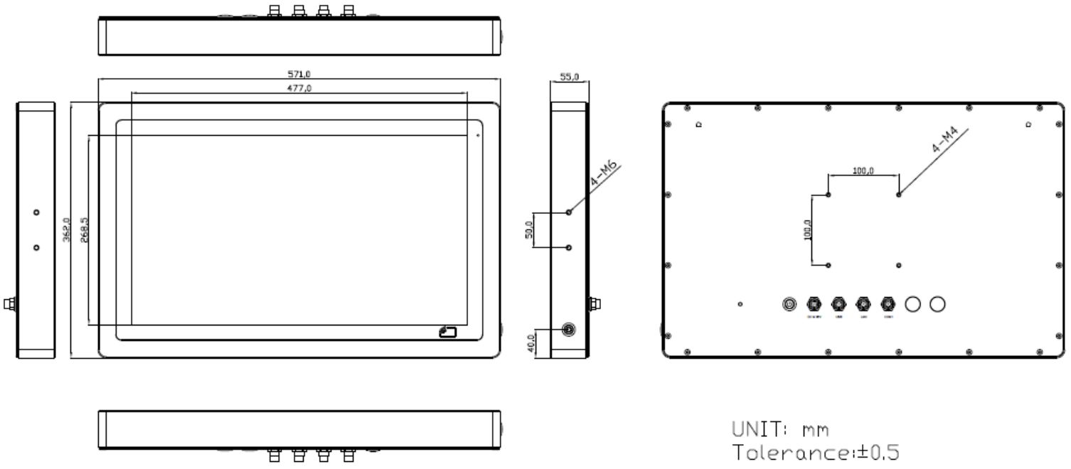
Figure 1.7: Dimensions of EX-91921V
