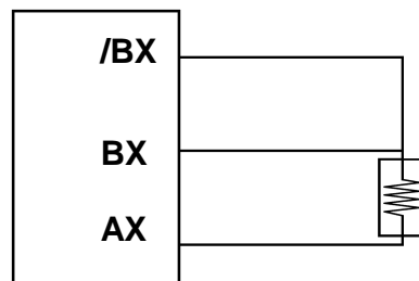
3-wire RTD connection
